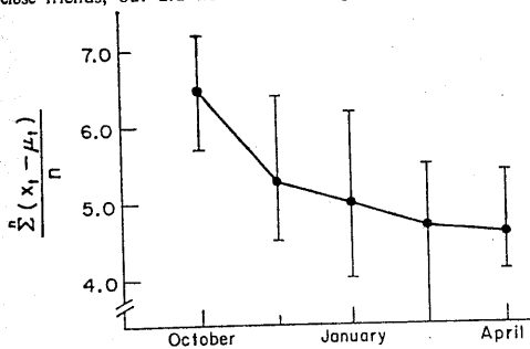
Fig. 1 The median individual mean difference from the group onset mean ( \frac{\sum (x_i - \mu_1)}{n} days) as a function of time. The asymptotic relation and non-overlapping confidence intervals 8 for the medians in October and late February, and October and April ( > 0.99 ), indicate an increase in synchrony for close friend groups.
